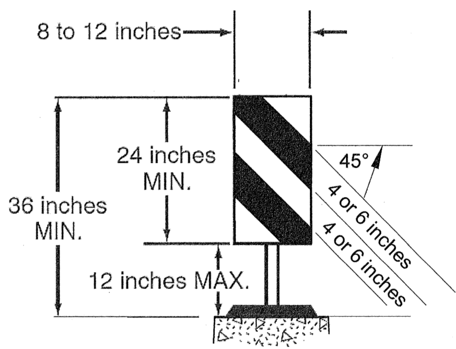
VERTICAL PANEL DETAIL SEE GENERAL NOTE 3, THIS SHEET.
