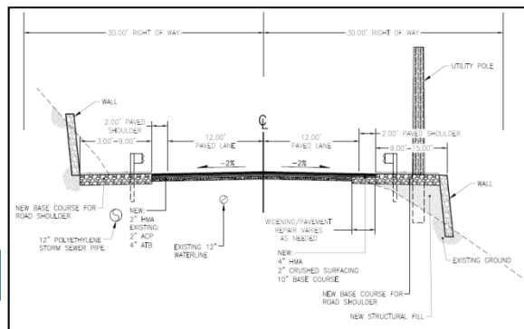
Proposed Section
