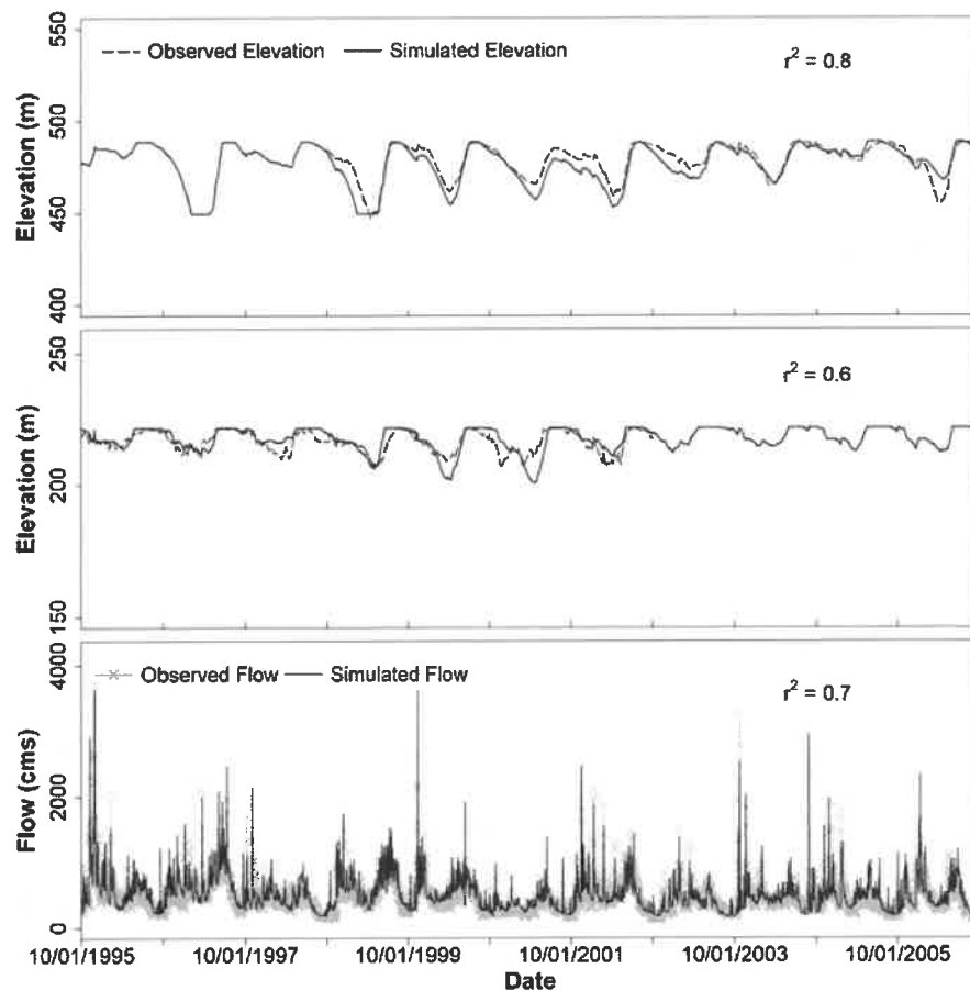
Figure 3. Time series of simulated and observed elevations at Ross dam (top) and Upper Baker dam (middle) and simulated and observed regulated flows at the Skagit River near Mount Vernon (bottom) for water years 1996–2006.
