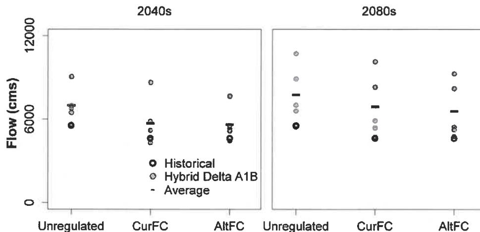
Figure 13. The magnitude of Q_{100} at the Skagit River near Mount Vernon for unregulated flows and for regulated flows under current flood control operations (CurFC) and alternative operations (AltFC) for the 2040s (left) and 2080s (right).
