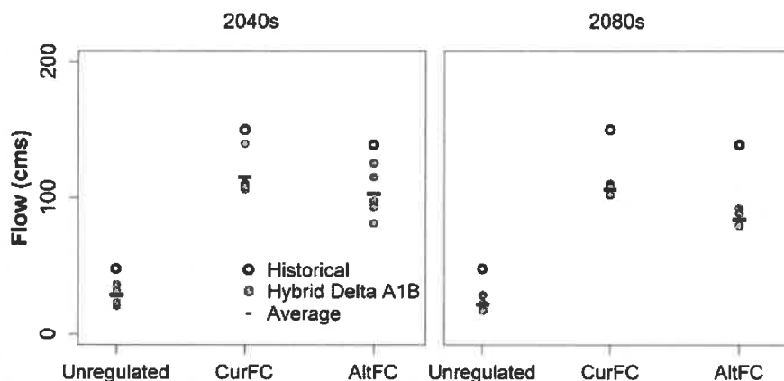
Figure 11. The magnitude of 7Q10 at the Skagit River near Mount Vernon for unregulated flows and for regulated flows under current flood control operations (CurFC) and alternative operations (AltFC) for the 2040s (left) and 2080s (right).
