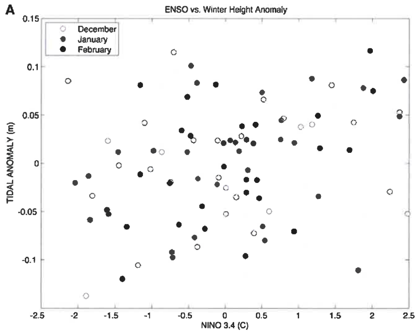
Figure 6. A) Relationship between the Nino 3.4 Index and mean monthly tidal anomaly for Seattle, WA (1970–1999). B) Observed Niño3.4 index (black line), 1950–2012, and ECHAM5 simulated transient Niño3.4 index values (gray line), 1970–2069.
