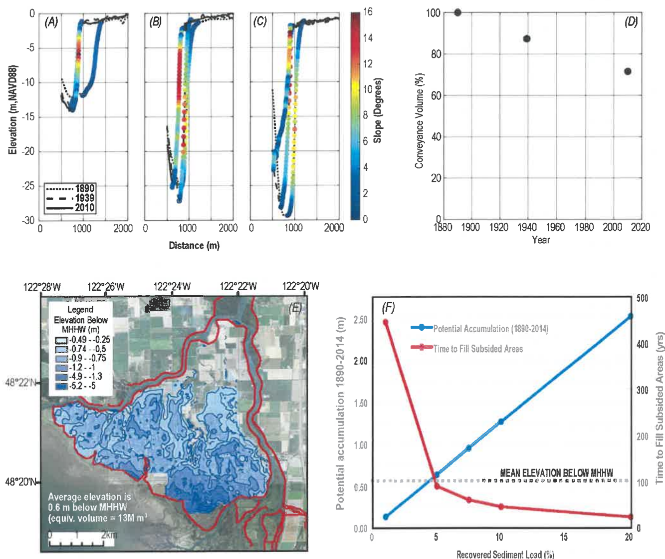
Fig. 12. Diagrams showing impacts of sediment export. (A-C) Plots showing the rapid steeping the delta front over time across transects 1-3 (Fig. 7) with unconsolidated sands vulnerable to failure. (D) Plot of the change in flow conveyance of central Skagit Bay in response to the delta progradation since 1890 (location in Fig. 4) showing a 22% reduction in the volume capacity for circulation and mixing. (E) Map showing the distribution of land surface elevations of Fir Island in 2014 ranging 0 to 5.2 m below Mean Higher High Water (mean = 0.6 m) associated with lost sediment supply and subsidence. (F) Plot of the potential vertical sediment accumulation over Fir Island that could have been gained between 1890 and 2014 (blue line) and the time in years in the future (red line) required to fill the equivalent volume of 13M m 3 associated with area 0.6 m below MHHW assuming up to 20% of the Skagit River sediment delivery to Fir Island. (For interpretation of the references to color in this figure legend, the reader is referred to the web version of this article.)
