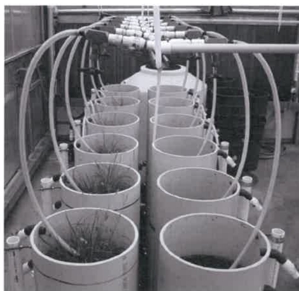
Fig. 1. The two sets of bioretention columns used to filter runoff from the September 2012 storm event. All columns contain a mixed layer of bioretention soil medium overlying a gravel aggregate drainage layer. The columns on the left are planted with Carex flacca .
