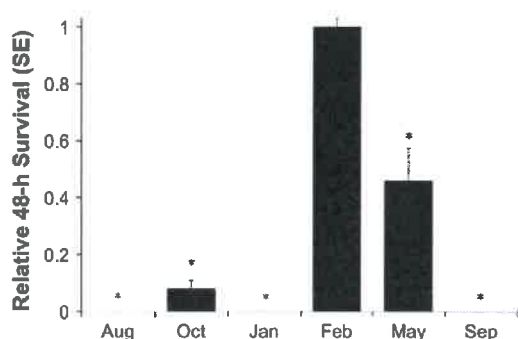
Fig. 2. Survival of C. dubia following 48-h exposure to first flush highway runoff relative to control survival for each storm event tested. Asterisks indicate runoff exposures that significantly affected survival relative to controls.
