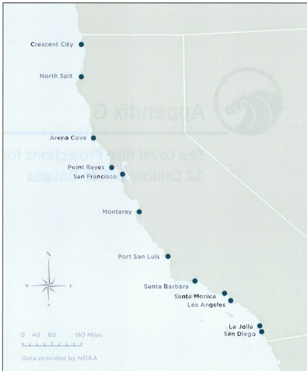
Figure G-1. Map of tide gauge locations (from OPC 2018)
