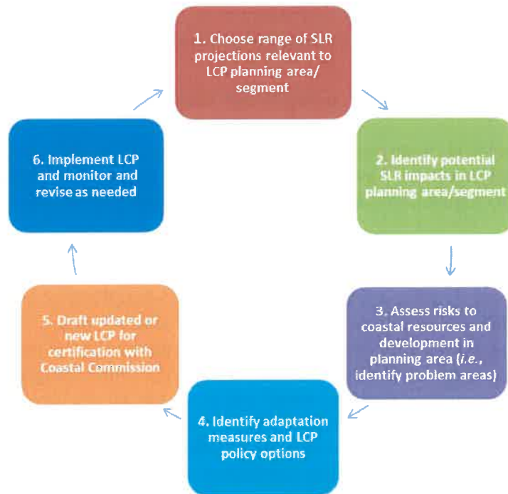
Figure 9. Sea level rise adaptation planning process for new and updated Local Coastal Programs
