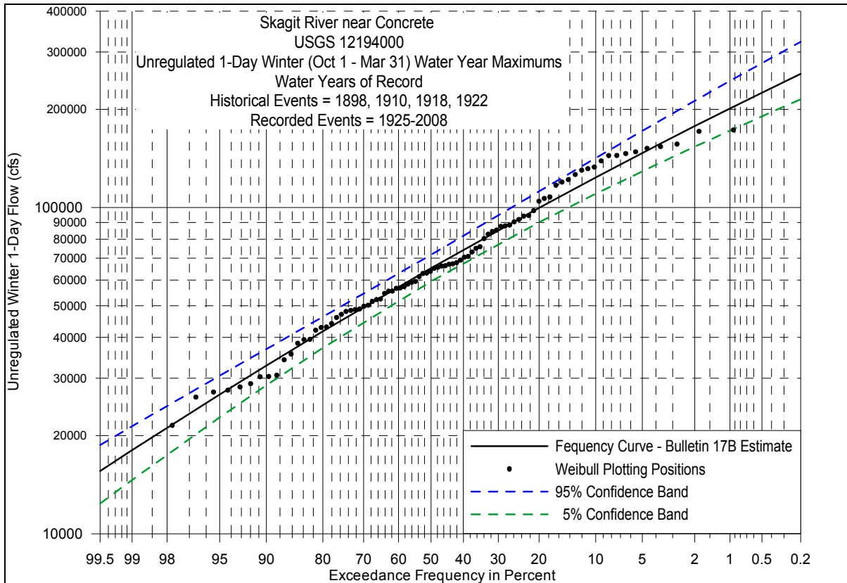
Figure 17. The unregulated one-day flow frequency curve and the confidence band together with all data used in the frequency analysis at Concrete
