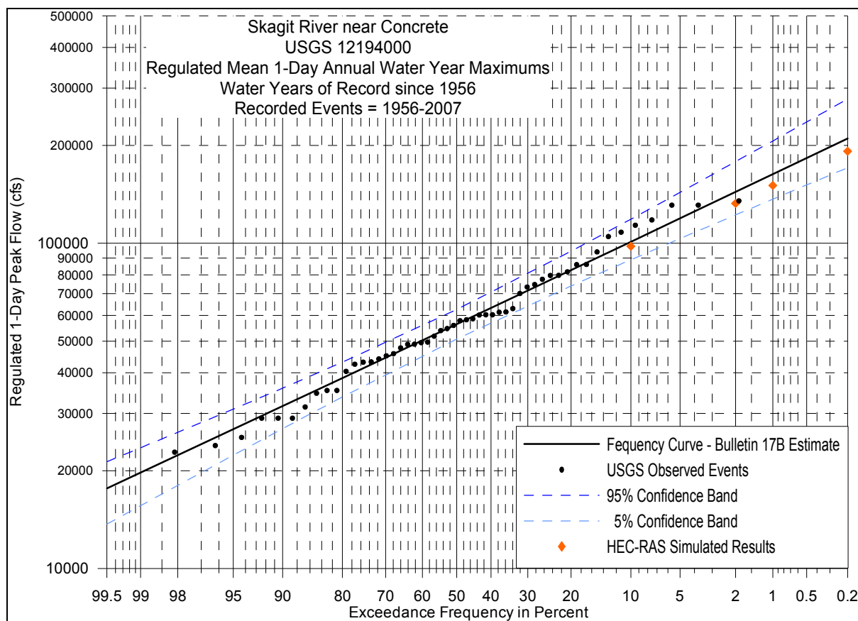
Figure 22. Flood frequency curve for regulated one-day discharges observed by USGS at Concrete, compared with the HEC-RAS simulated regulated one-day flows at Concrete for the 10-, 50-, 100-, and 500-year synthetic events
