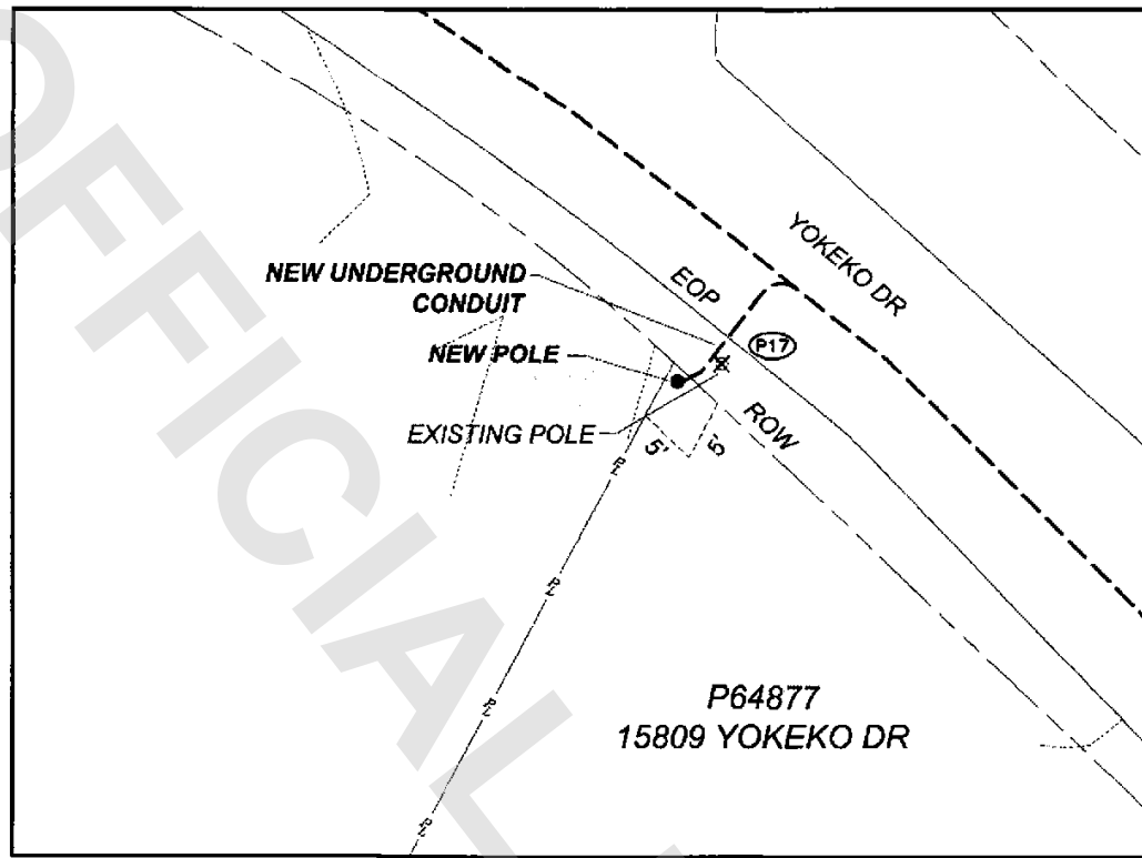
EASEMENT DETAIL (P64877)
