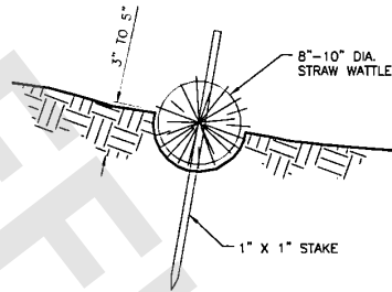
STRAW WATTLE DETAIL NOT TO SCALE
