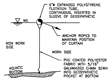
TURBIDITY CURTAIN NOT TO SCALE
